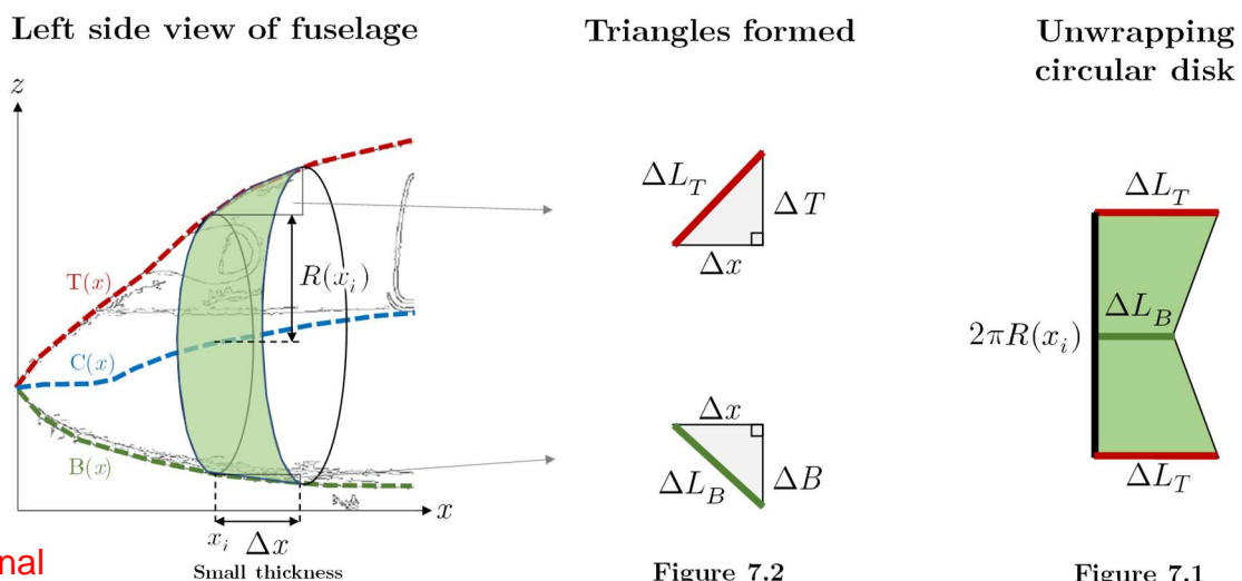
Figure 7. The calculation of the surface area of the fuselage.
