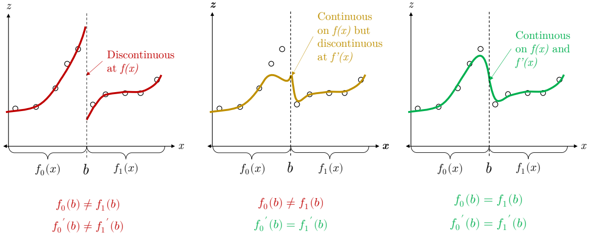
Figure 12. Demonstrations of discontinuities in f(x) when f_k(b) \neq f_{k+1}(b) and f_k'(b) \neq f_{k+1}'(b) .
